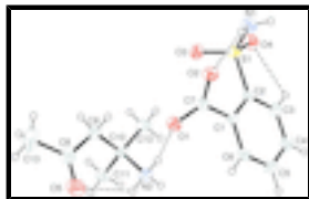
Fig. 1. View of the title compound with the atom numbering scheme. The thermal ellipsoids are drawn at the 30% probability level. H-atoms are shown by small circles of arbitrary radii. Intramolecular H-bonds are shown by dotted lines.
