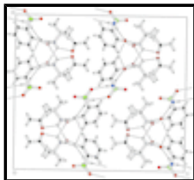
Fig. 2. The partial packing ( PLATON ; Spek, 2009) which shows that molecules form dimers of 2-sulfamoylbenzoate and connected to 2-methyl-4-oxopentan-2-aminium through intermolecular H-bondings.
